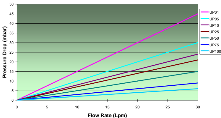
Flow Rate/Pressure Drop Water, 10" Element
